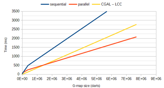
Figure 8: Execution time for Menger sponge rule.
