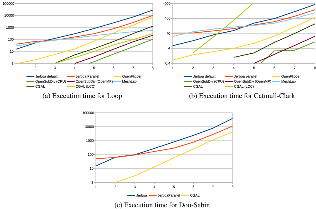
Figure 7: Execution time for subdivision operations.
