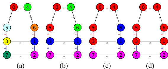
Figure 4: Execution of the Islet algorithm for orbit type \langle \alpha_0, \alpha_1 \rangle .
