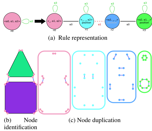
Figure 2: Catmull-clark subdivision operation in Jerboa.
