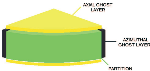
Fig. 3 The positioning of ghost layer points
