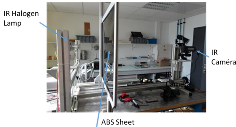
Fig.2. Experimental setup
