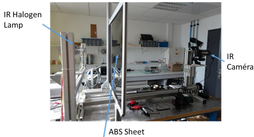
Fig.2. Experimental setup
