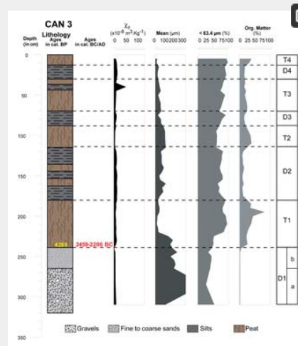
Fig 4. Core profile of CAN 3 borehole where sedimentological results and environments are presented. Magnetic susceptibility measurement at low frequency, LASER grain size and organic matter content. https://doi.org/10.1371/journal.pone.0226358.g004
