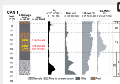
Fig 6. Core profile of CAN 1 borehole where sedimentological results and environments are presented. Magnetic susceptibility measurement at low frequency, LASER grain size and organic matter content. https://doi.org/10.1371/journal.pone.0226358.g006
