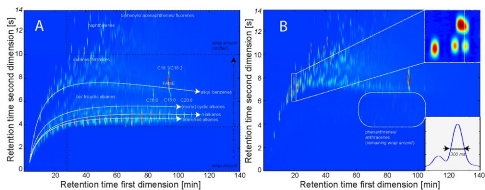
Fig. 10 Application of spectral filters for different petrochemical matrixes. (A) GC×GC-VUV chromatogram of a diesel fuel (total VUV-absorption 125-240 nm). (B) Application of 170-200 nm filter to (A) for the discrimination of \pi^* \leftarrow \pi chromophores. Reprinted with permission from [40] Copyright (2016) American Chemical Society.
