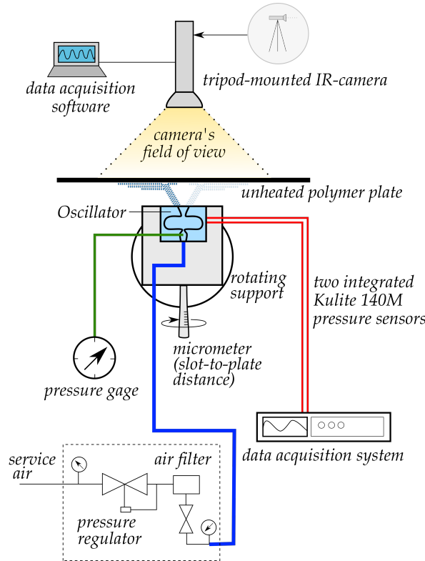
Figure 3: Setup of the preliminary experiment with an unheated polymer plate.
