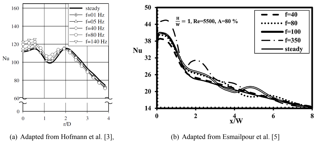
Figure 1: Nusselt number profile along heated plates cooled by means of steady and periodically excited jets impinging from close distances, showing the typical secondary and tertiary peaks associated with small standoff distances and unsteady jets respectively.
