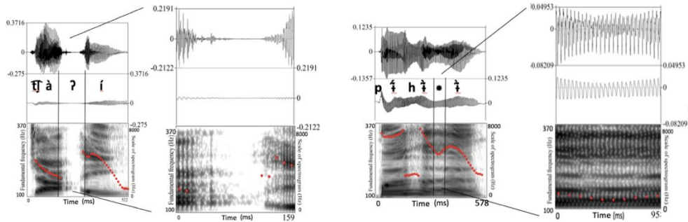
Figure 6: Sound, EGG and Spectrogram for words 'tiger' [tʃãʔi] and 'sit down-M.PR.IMP' [pìhì*ɕ]. Male
