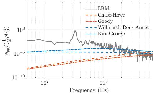
Figure 11. Wall pressure fluctuation spectrum \phi_{pp} at the trailing edge, mid-span of the optimized blade from LBM simulations and numerical models.
