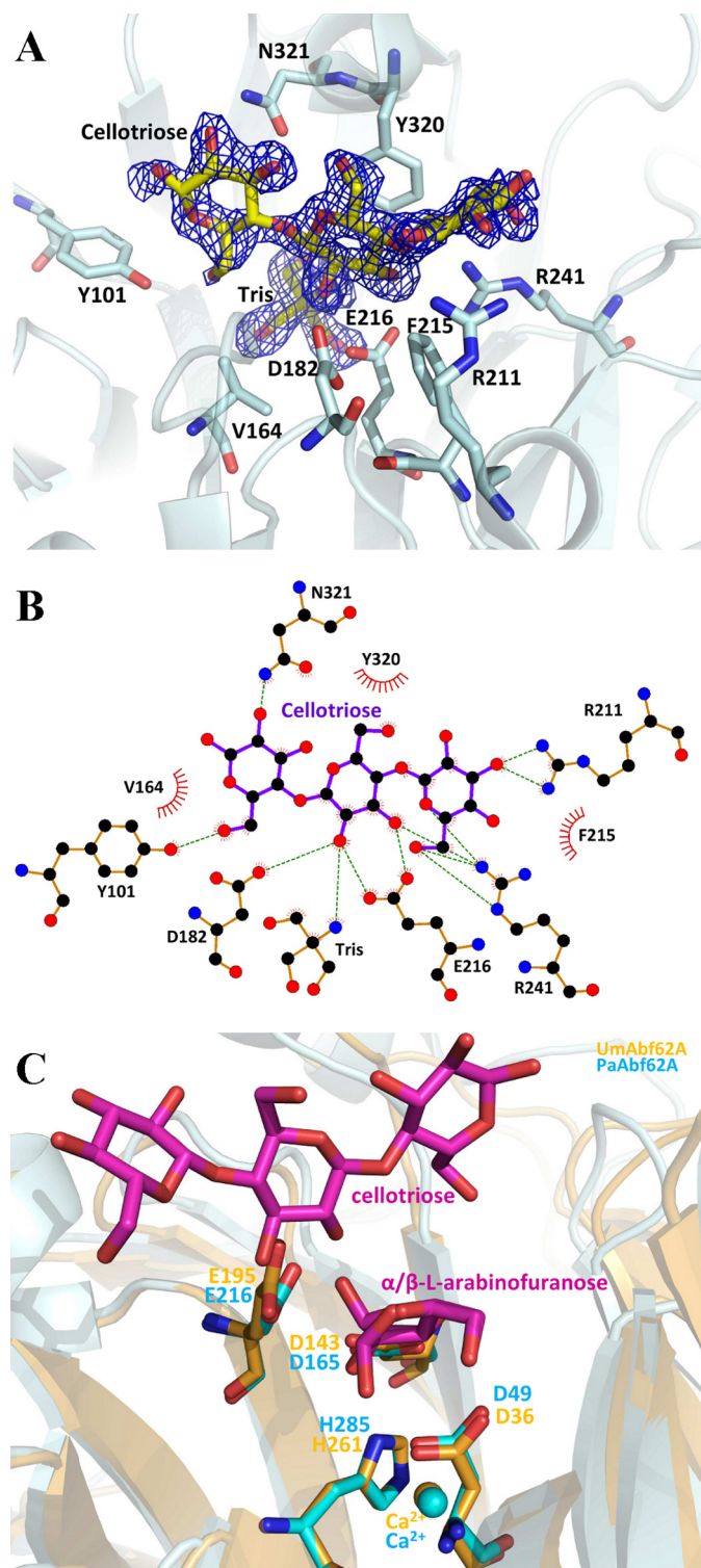
FIGURE 7. PaAbf62A in complex with cellotriose. A , structure of cellotriose in the active site pocket of PaAbf62A . Sugar is displayed as stick and protein as a schematic. Catalytic amino acids are named using the one-letter code of the amino acid followed by the position in the sequence. The electron density is displayed in dark blue and has been contoured to 1\sigma . B , schematic diagram showing hydrogen-bonding, water-bridged, and hydrophobic interactions between PaAbf62A and cellotriose. Amino acid residues of PaAbf62A that have hydrophobic interactions with cellotriose are shown as spiked spheres (with distances of less than 3.5 \text{ \AA} ). Direct and water-bridged hydrogen-bonding interactions are indicated by dashed lines . C , superimposition of complex structures of PaAbf62A and UmAbf62A sugar are colored in magenta , UmAbf62A is colored in gold , and PaAbf62A is colored in cyan .
