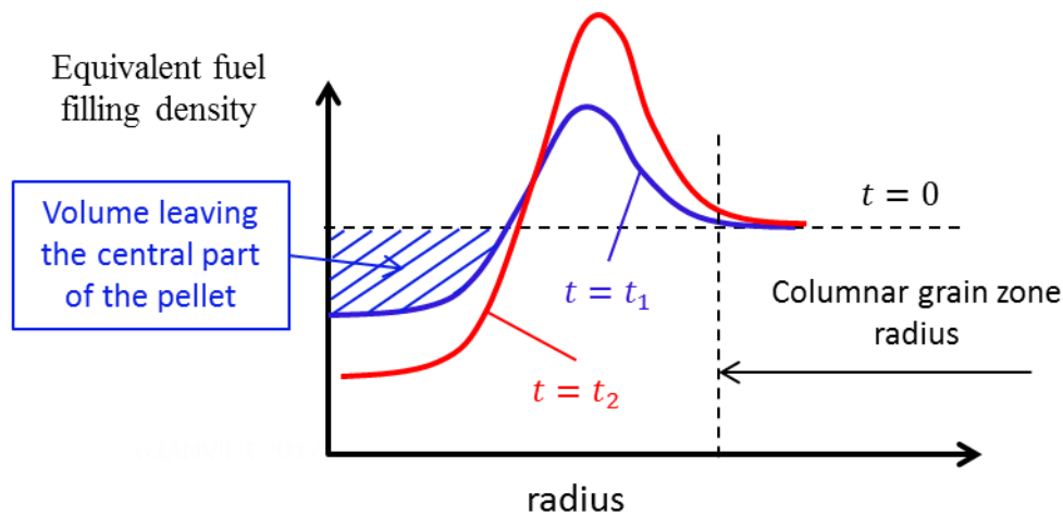
Figure 4 : Computation of the fuel volume transferred according 1D results of GERMINAL. Secondly, a displacement boundary condition is added in the 3D single fragment finite element model to compute the radial relocation displacement induced by the mass transfer. This boundary condition (see Figure 5) is defined on the free surface of the pellet fragment for the columnar grain zone (blue line in Figure 5) with a unilateral condition where e(t) is the half thickness of the transferred volume between two pellet fragments at time t .
