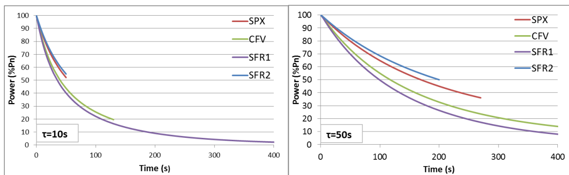
FIG. 8. Power for ULOSSP transient
