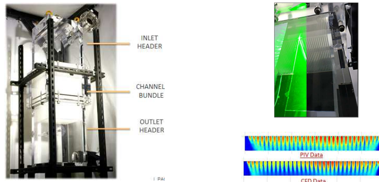
Fig.4 : DANAH facility. Illustration showing calculated and measured channels outlet velocity profiles [4].
