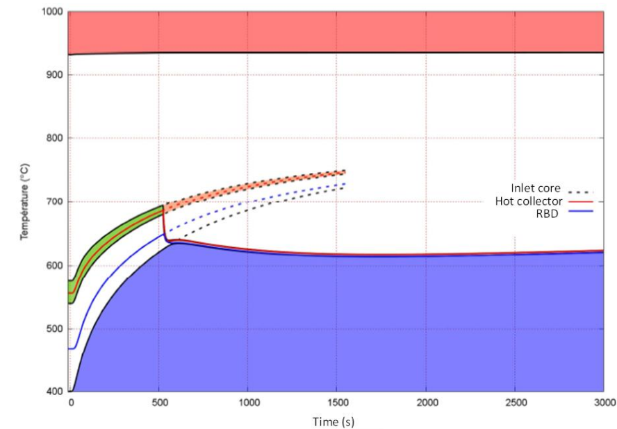
FIG. 4 : Temperature during an ULOHS
