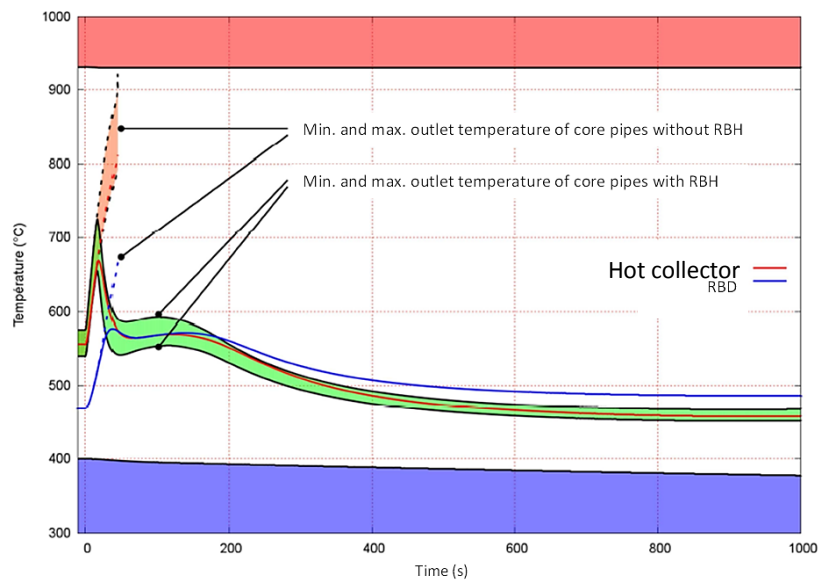
FIG. 3 : Na temperature during ULOF/PP
