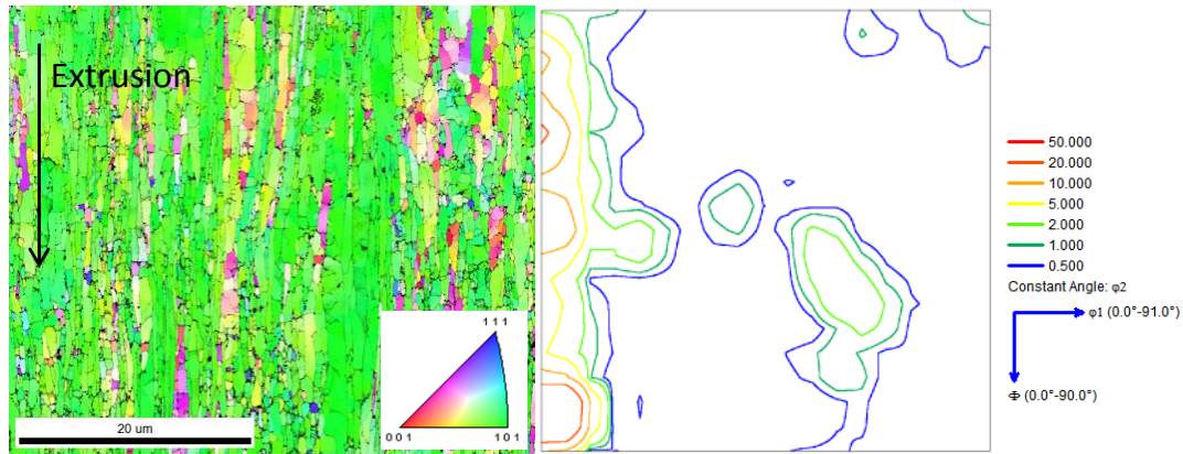
FIG. 2: IPF maps showing crystal direction parallel to extrusion direction and corresponding ODF section plot at \varphi_2 = 45^\circ after annealing 1h at 1300^\circ\text{C}
