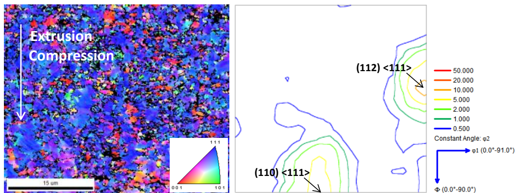
FIG. 4: IPF maps showing crystal direction parallel to compression direction and corresponding ODF section plot at \phi_2 = 45^\circ after uniaxial compression
