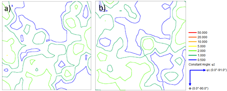
FIG. 6: ODFs section plot at \phi_2=45^\circ after compression and annealing 1h at (a) 1150°C and (b) 1300°C
