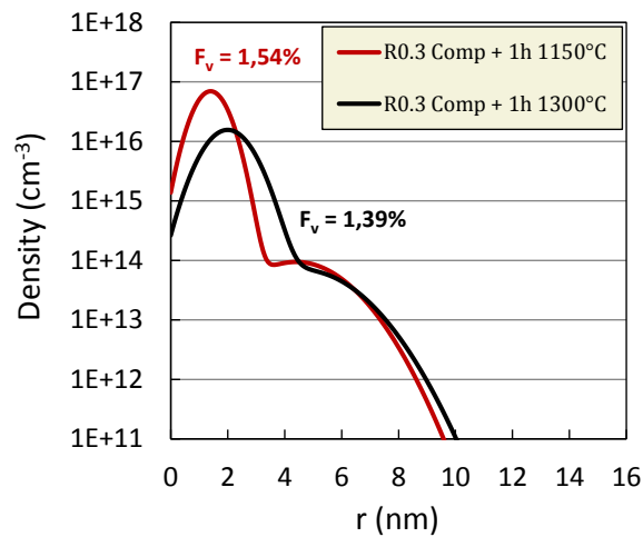
FIG. 8: Nano-particles size distributions after compression and annealing
