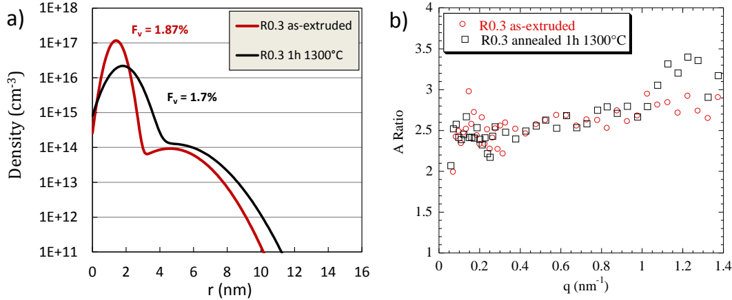
FIG. 3: (a) Nano-particles size distributions and (b) A ratio as extruded and after 1h at 1300°C
