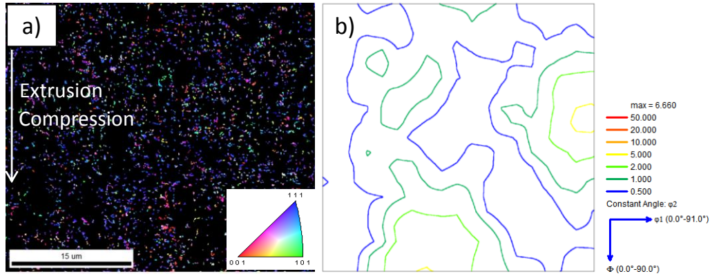
FIG. 9: (a) IPF map showing crystal direction parallel to compression direction for subgrains smaller than 0.25 \mu\text{m} and (b) corresponding ODF section plot at \phi_2 = 45^\circ
