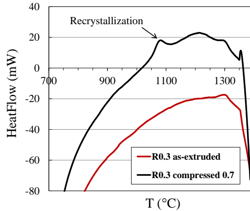
FIG. 7: Heating part of DSC curves for the as-extruded and deformed grades
