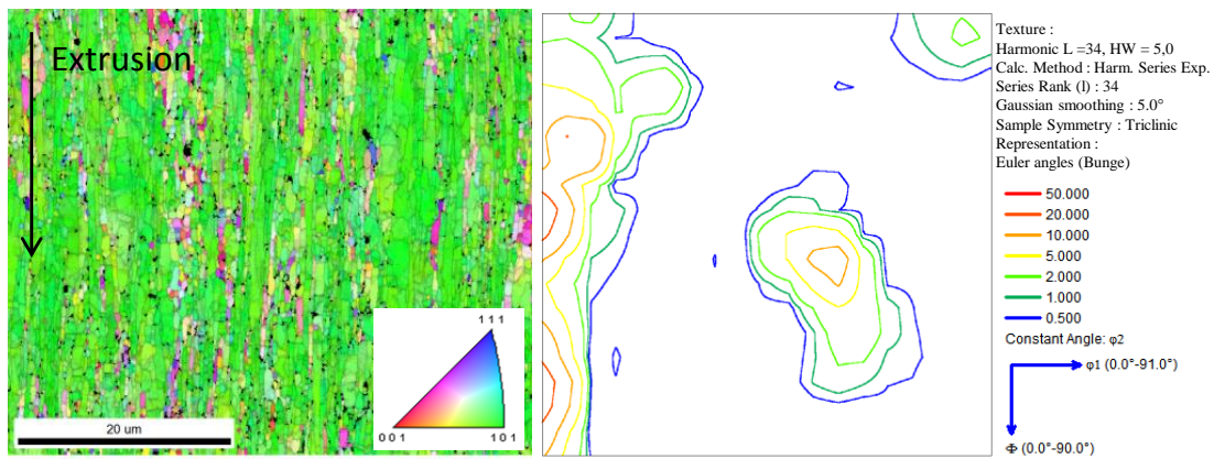
FIG. 1: IPF maps showing crystal direction parallel to extrusion direction and corresponding ODF section plot at \varphi_2 = 45^\circ for the as-extruded material
