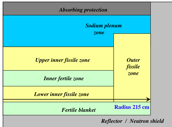
Fig. 9. Section of the ASTRID CFV-V1 core (1500 MWth)
