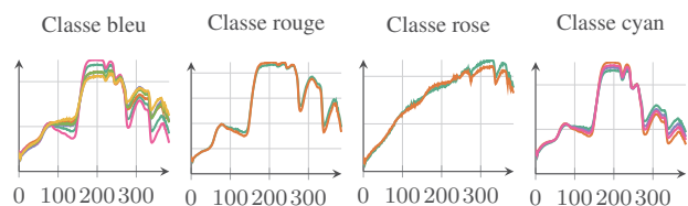
FIGURE 3 – Centroïdes spectraux des différents clusters pour chaque classe. [1] A. Villa, J. Chanussot, J. A. Benediktsson, and C. Jutten, "Spectral unmixing for the classification of hyperspectral images at a finer spatial resolution," IEEE J. Sel. Top. Signal Process. , vol. 5, no. 3, pp. 521–533, 2011. [2] A. Lagrange, M. Fauvel, S. May, and N. Dobigeon, "Hierarchical Bayesian image analysis : From low-level modeling to robust supervised learning," Pattern Recognit. , vol. 85, pp. 26–36, 2019.
