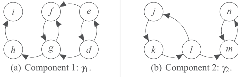
Fig. 2. Connected components resulting from the grounded removal pre-processing.
