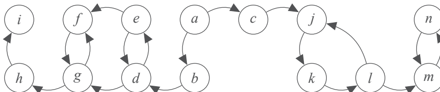
Fig. 1. Example of an argumentation framework AF.
