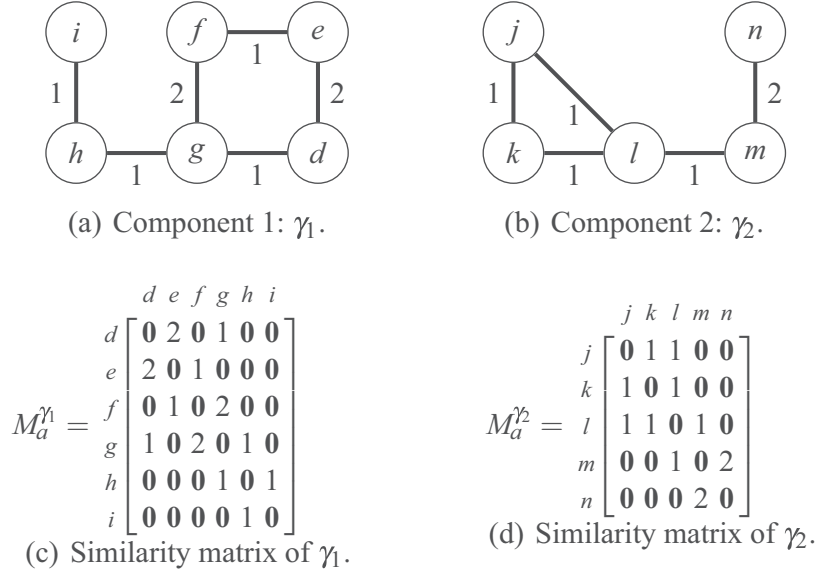
Fig. 3. Step 1 of the spectral clustering.
