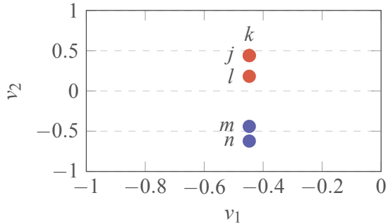
Fig. 6. Step 4 of the spectral clustering.
