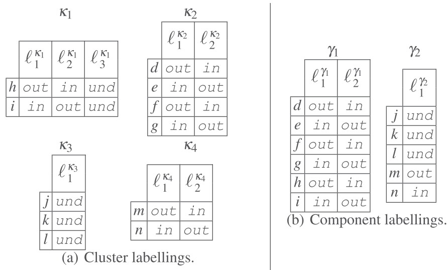
Fig. 8. Labellings computed using our algorithm.
