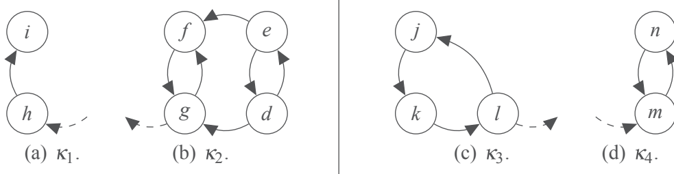
Fig. 7. Identified clusters.
