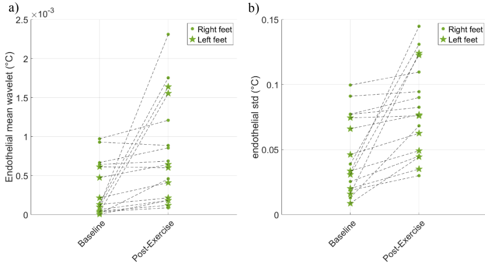
Figure 10: Indicator variations for a healthy volunteer's signal, filtered within the endothelial range. a) mean wavelet value \bar{W}_{iaJa}^{endo} , b) standard deviation std_{iaJa}^{endo} . Dotted lines indicate, for each subject, variations in the indicator after exercise.
