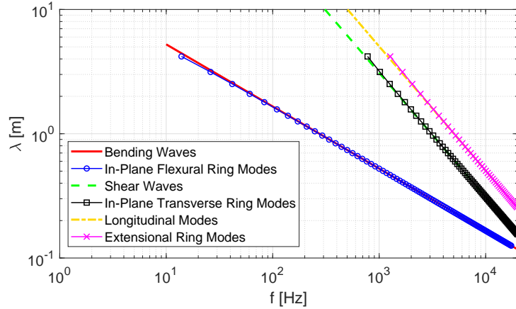
Figure 3: Bending, shear and longitudinal wavemodes wavelength in an infinite beam and the corresponding beam-ring circumferential modes
