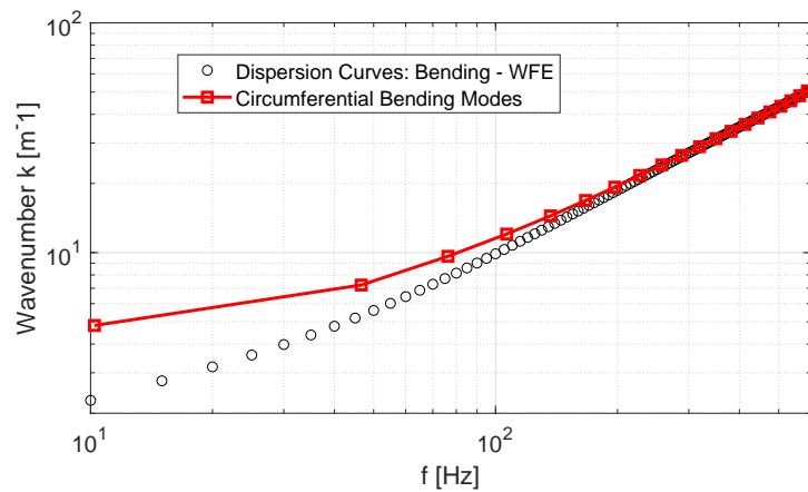
Figure 20: Bending Waves for the double-wall panel with mechanical connection. Numerical comparison between the WFEM and the present analogy.
