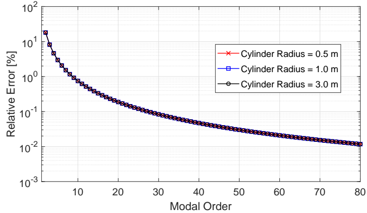
Figure 4: Relative error (log-scale) between the bending wavelength in an infinite panel and the modal wavelengths of an infinite cylinder
