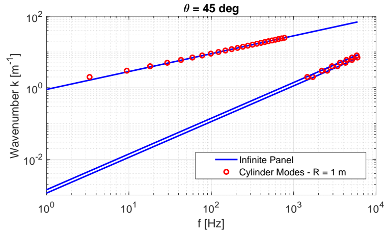
Figure 14: Dispersion curves of the laminate panel; heading angle 45^\circ . CLPT results used as a reference.
