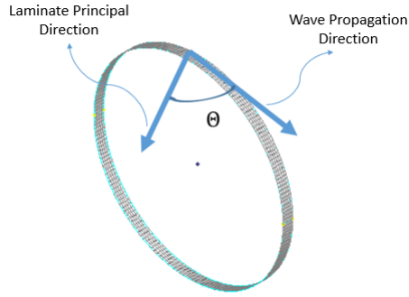
Figure 11: Scheme of the laminate heading angle with respect to the wave propagation direction.
