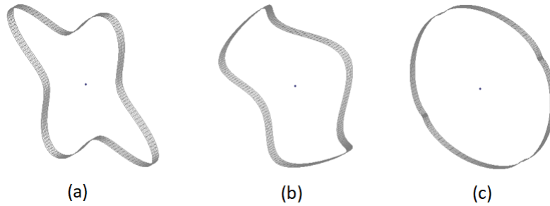
Figure 17: Purely circumferential modes in a laminate infinite panel; X-Y as cross sectional plane. Fourth circumferential mode - (a) Bending: 16.6 Hz; (b) Shear: 1364 Hz; (c) Longitudinal: 4674 Hz
