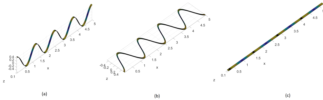
Figure 18: Rectified circumferential modes in a laminate infinite panel; X-Y as cross sectional plane. Fourth circumferential mode - (a) Bending: 16.6 Hz; (b) Shear: 1364 Hz; (c) Longitudinal: 4674 Hz
