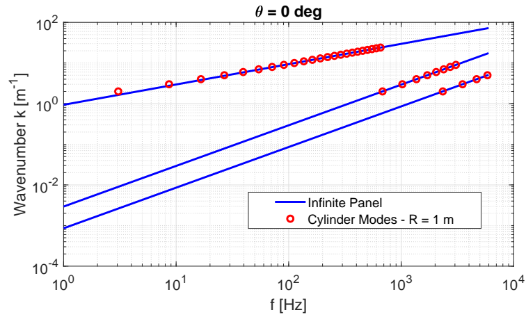
Figure 12: Dispersion curves of the laminate panel; heading angle 0^\circ . CLPT results used as a reference.
