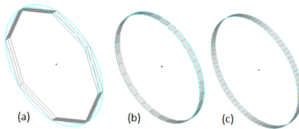
Figure 8: Comparison for increasing number of elements for a given circumference radii R . From the left side: 8, 32, 80 elements
