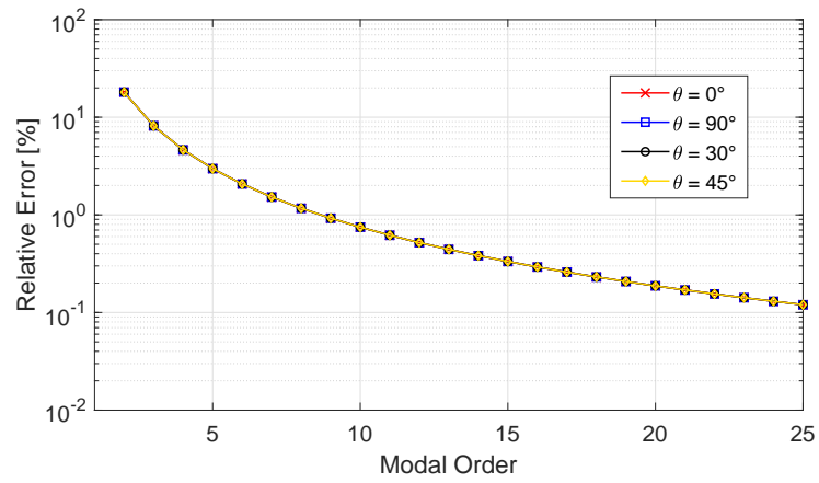
Figure 15: Relative errors (log-scale) for different heading angles (bending waves). The CLPT results used as reference.
