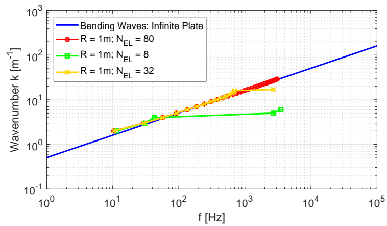
Figure 9: Effect of the mesh: comparison for increasing number of elements for a given circumference radii R (isotropic panel). Elements size variable.
