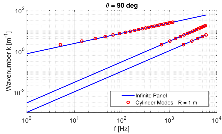
Figure 13: Dispersion curves of the laminate panel; heading angle 90^\circ . CLPT results used as a reference.
