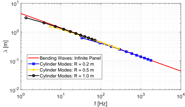
Figure 6: Isotropic uniform plate: infinite panel solution and the circumferential modes of a cylindrical finite structure made of plate elements
