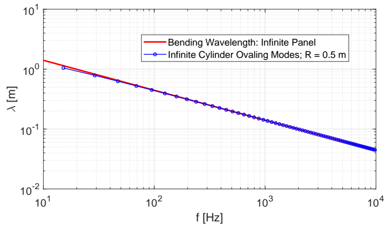
Figure 5: Bending wavelength in an infinite panel and the ovaling modes of an infinite cylinder
