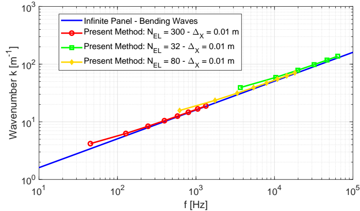
Figure 10: Effect of the mesh: comparison for increasing number of elements for a given element size (isotropic panel). Circumference radii R variable: Fig. 7(a) 0.05 m, Fig. 7(b) 0.13 m, Fig. 7(c) 0.48 m
