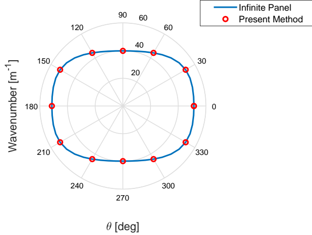
Figure 16: Pattern of the bending wavenumbers for the laminate plate analysed; 3000 Hz
