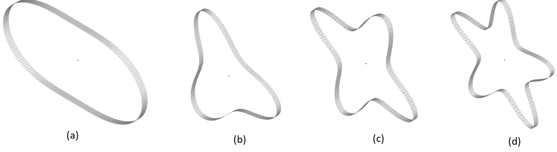
Figure 2: Purely circumferential bending modes in a circular structure: (a) Circumferential Order = 2; (b) Circumferential Order = 3; (c) Circumferential Order = 4; (d) Circumferential Order = 5.
