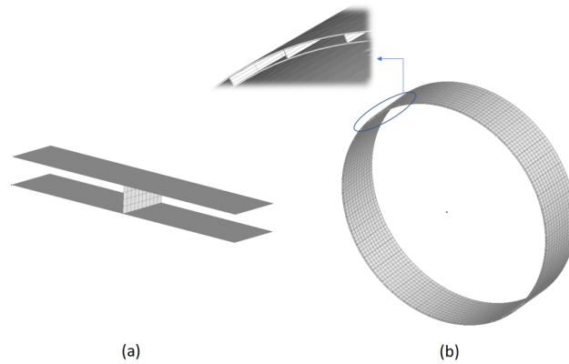
Figure 19: A double-wall panel with mechanical connection: (a) Elementary FE Cell; (b) Cylindrical Model.
