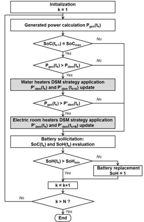
Fig. 6. General flowchart of the multi-source system simulation, including DSM strategies
