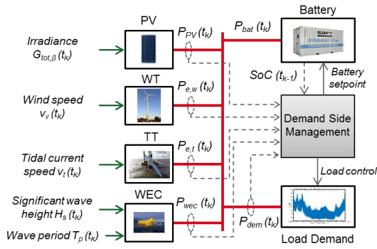
Fig. 1. Overview of the considered multi-source system model
