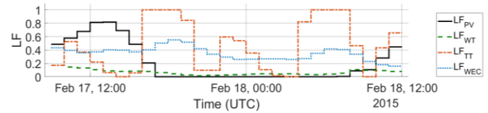
Fig. 11. Hourly load factor of each source
