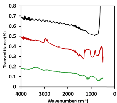
Figure 1. Fourier transformed infrared spectra obtained for Macro-bare electrode (upper black curve), grafted propargyl Br electrode Macro-Br (lower green curve), and grafted ethynyl Fc electrode Macro-Fc (red curve, in the middle).
