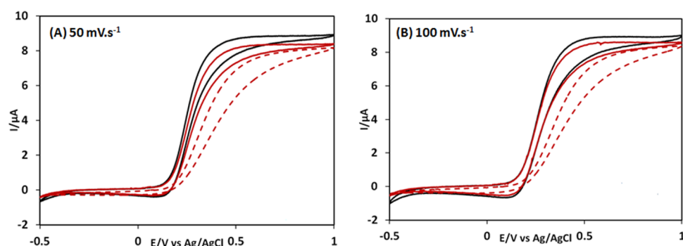
Figure 3. Cyclic voltammetry recorded at ultra-microelectrodes for ferrocyanide ( 2 \times 10^{-3} M) oxidation, in water containing 0.5 M KCl as the electrolyte and Ag/AgCl as the reference electrode, at different scan rates of (A) 50 and (B) 100 \text{mV s}^{-1} . Different electrodes were studied: bare glassy carbon electrode (black), Macro-Br after 2 h of reaction (red), and Macro-Br after 24 h of reaction (dashed red).
