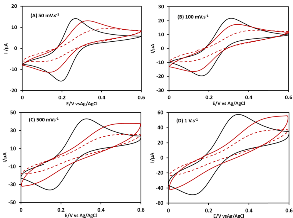
Figure 2. Cyclic voltammetry recorded at a 1.4 mm diameter glassy carbon millimetric electrodes in an aqueous electrolyte (0.5 M KCl) containing ferri/ferrocyanide ( 2 \times 10^{-3} M) and Ag/AgCl as the reference electrode, at different scan rates of (A) 50, (B) 100, (C) 500, and (D) 1000 \text{mV s}^{-1} and different surface conditions. Bare glassy carbon electrode (black), Macro-Br after 2 h of reaction (red), and Macro-Br after 24 h of reaction (dashed red).
