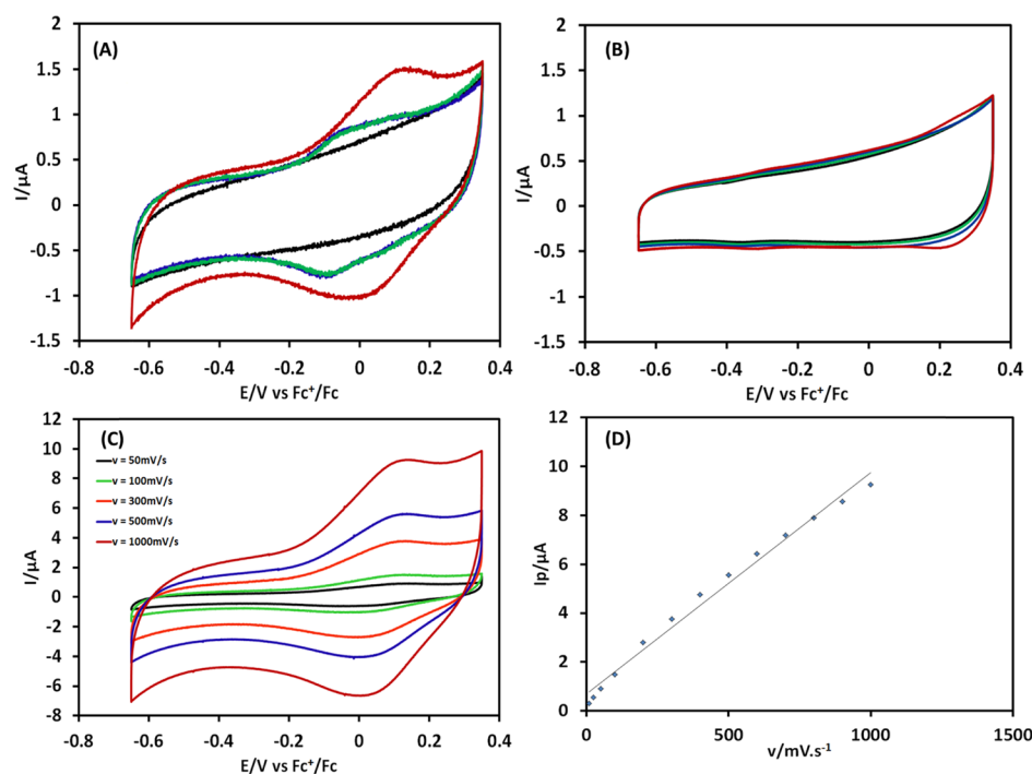
Figure 4. (A) Cyclic voltammetry on millimetric electrodes of ferrocene grafted onto the electrodes in ACN containing 0.5 M \text{LiClO}_4 at different states of the surface. Bare glassy carbon electrode (black), Macro-Fc after 30 min of reaction (blue), Macro-Fc after 2 h of reaction (green), and Macro-Fc after 24 h of reaction (red). Scan rate: 100 \text{mV s}^{-1} . (B) Cyclic voltammetry on the millimetric bare electrode, which is immersed in a solution containing ferrocene in toluene for 30 min, 2 h, and 24 h before starting the CV. Scan rate: 100 \text{mV s}^{-1} . (C) Cyclic voltammetry of ferrocene grafted after 24 h of reaction on the surface at different scan rates. (D) Values of the oxidation peak intensity for CV (C) as a function of scan rate values.
