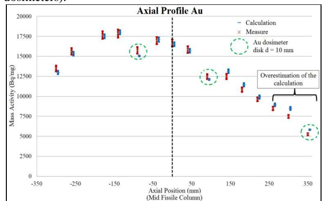
Fig. 6. Au dosimeters of the North East plate – axial mass activity distributions – measurements and calculations
