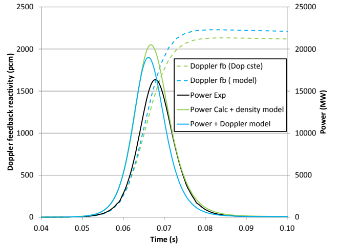
Fig. 8. Effect of Doppler model on transient of power calculation
