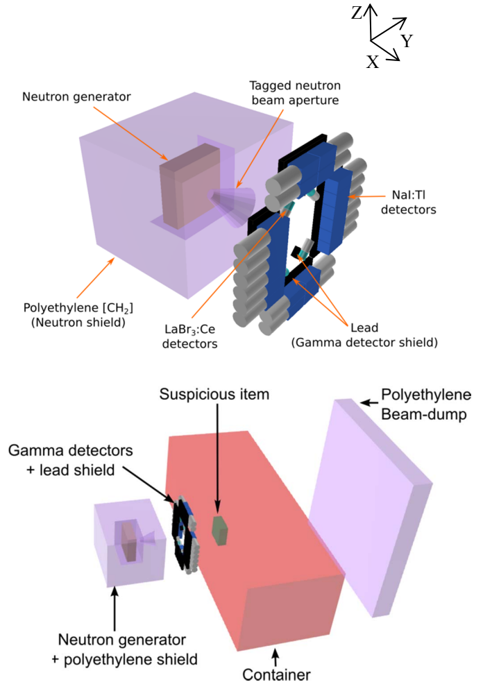
Fig. 2. General 3D view of the RRTNIS.
