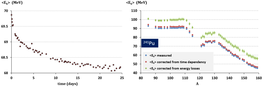
Figure 4. On the left, the evolution over time of the measured post-neutron mean kinetic energy for the mass 136 at the ionic charge 23. On the right, the measured post-neutron mean kinetic energy as a function of the fission product mass before (in blue) and after correction of the energy dependency to time (in red) and after correction from the energy loss in the Pu and the Ni protective foil (in green).
