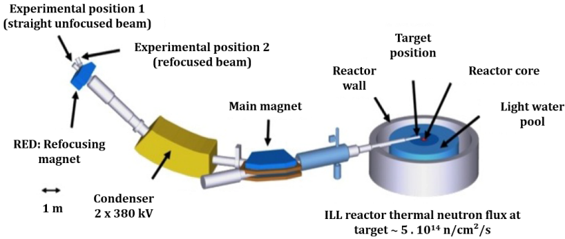
Figure 1. The Lohengrin mass spectrometer at the ILL, Grenoble. The ILL high neutron flux compensates the small geometrical acceptance of the instrument.
