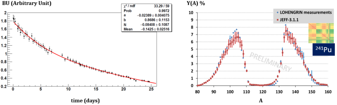
Figure 3. On the left, the time evolution of the fissile material quantity in the target, so-called Burn-Up (BU). On the right, the ^{241}\text{Pu} isobaric fission yields measured at Lohengrin (in blue), and the experimental covariance matrix, compared to JEFF-3.1.1 (in red). Lohengrin measurements are normalized to 1 for the heavy peak. These results are combining two experiments, the first one performed in 2013 [10] and the second one in 2015 [11].
