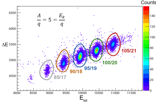
Figure 2. Raw results from the ionization chamber for the ratio A/q = 5 and E_k/q = 5 . The total count rate for each mass can be measured unambiguously with sufficient statistics.
