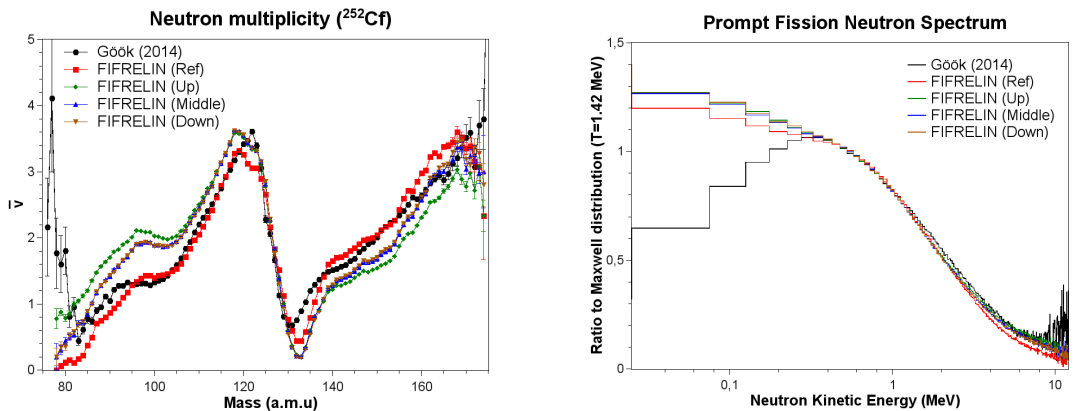
Figure 3. Comparison of the sawtooth (left) and PFNS (right) for the four simulations and experimental data [13].
