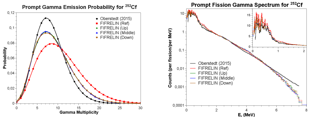
Figure 4. Comparison of the gamma multiplicity distribution (left) and PFGS (right) for the four simulations and experimental data [10].
