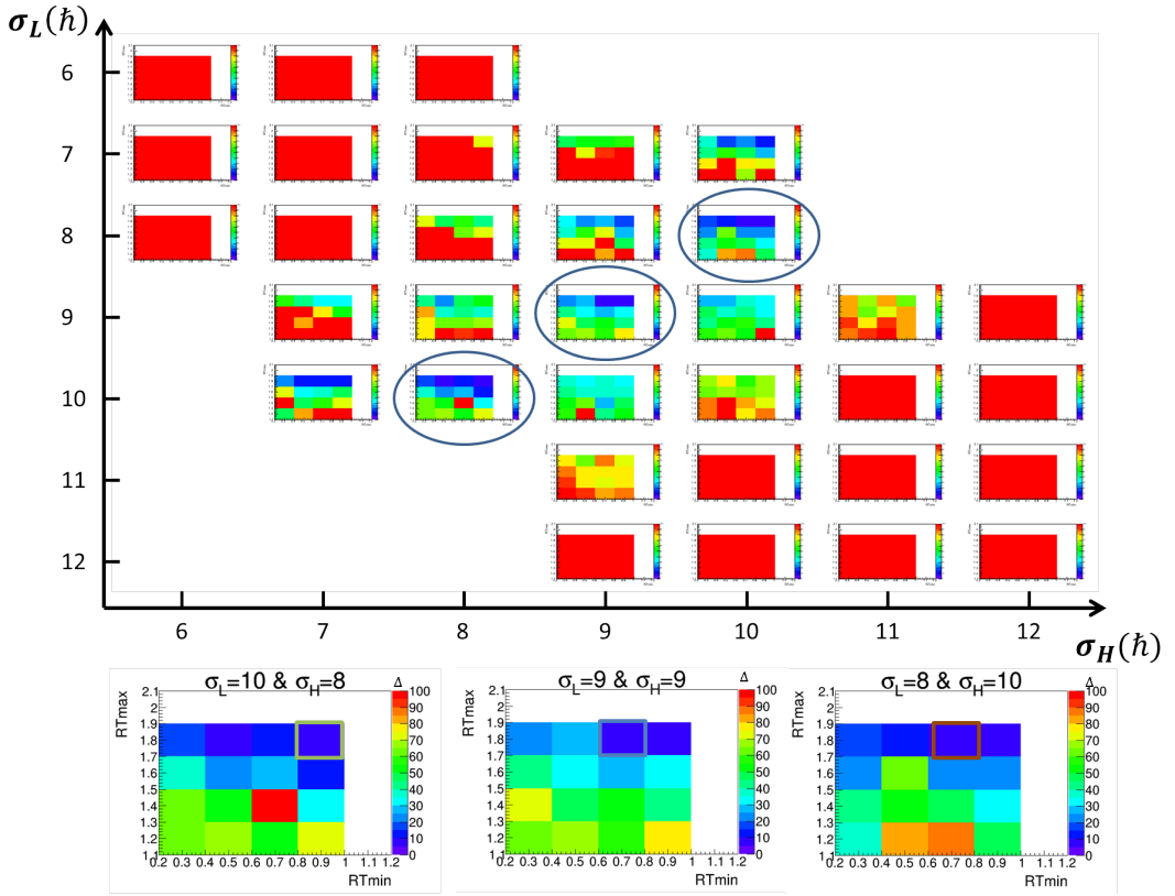
Figure 2. Comparison of \bar{\nu} and \overline{M}_\gamma from simulations and experimental data. 528 simulations of input parameters ( RT_{\min} , RT_{\max} , \sigma_L , \sigma_H ) were performed. Warmer the color is, worst the difference with experimental data is. The best cases are plotted in the lower part of the figure.
