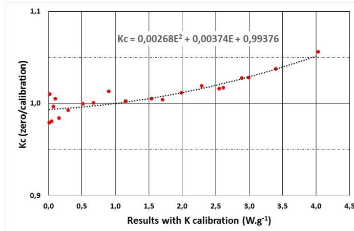
Fig. 8 – Results obtained by the zero and the calibration methods in upper part of the core up to 4 \text{ W.g}^{-1} . Measurement of the K_c correction factor.
