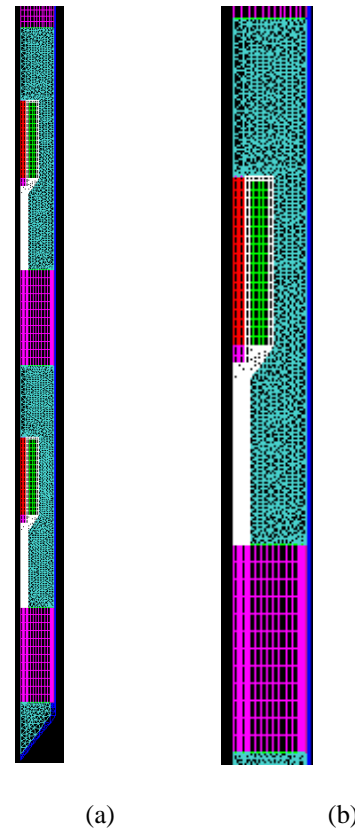
Fig.4 - CALMOS2 meshing of the probe (a), zoom on the reference cell (b)
