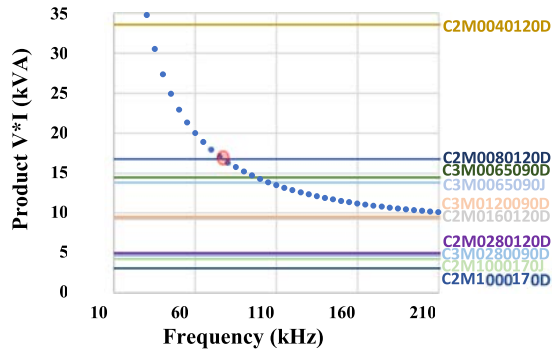
Fig. 7. Selection of the switches via the V I product.
