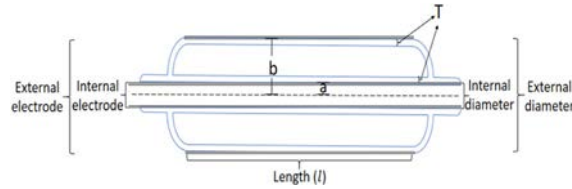
Fig. 1. DBD lamp geometry.
