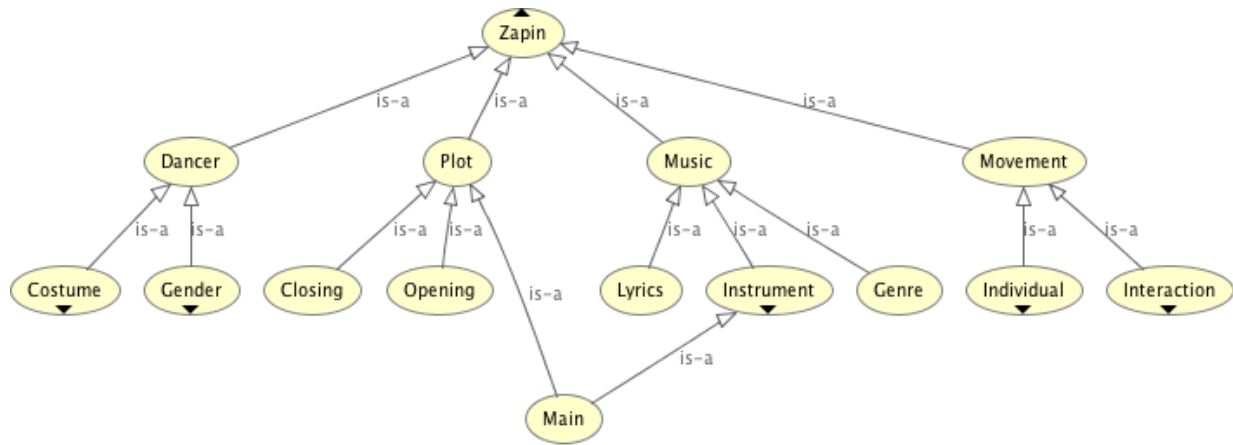
Fig. 1: Overview of the proposed Zapin Ontology
