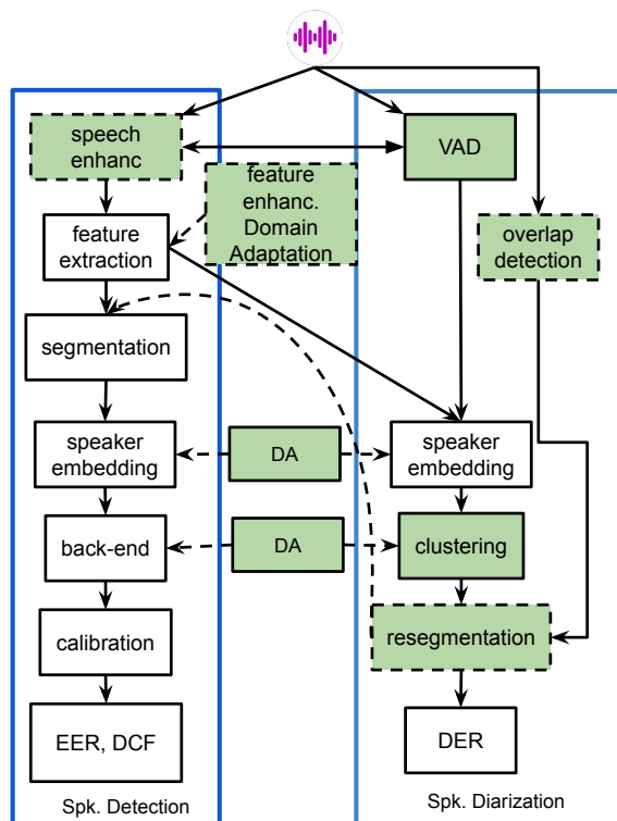
Fig. 1. Speaker detection pipeline. \square is the baseline system, \square are the new parts that are included in the pipeline, shaded- \square are the modules that were investigated.
