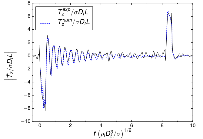
Fig. 23 Comparison of the filtered torque and the computed torque in the z-direction throughout time for manoeuvre n°1
