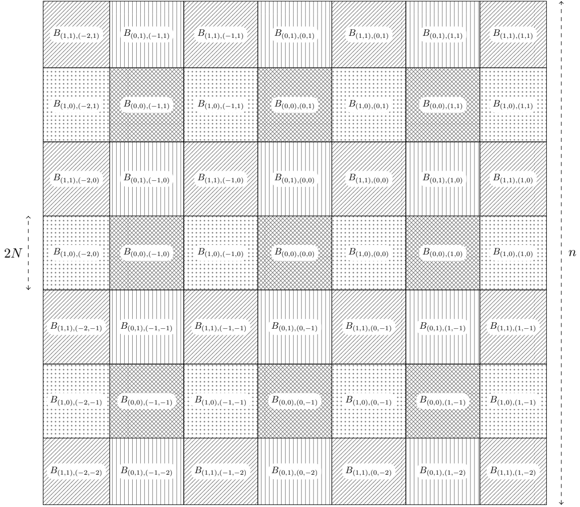
Figure 9: Partition of \Lambda(n) in 2^d subsets \mathcal{D}_x each corresponding to a hatching pattern, and each \mathcal{D}_x being in turn partitioned into boxes \mathcal{B}_{x,y} with y \in \Lambda(M) .
