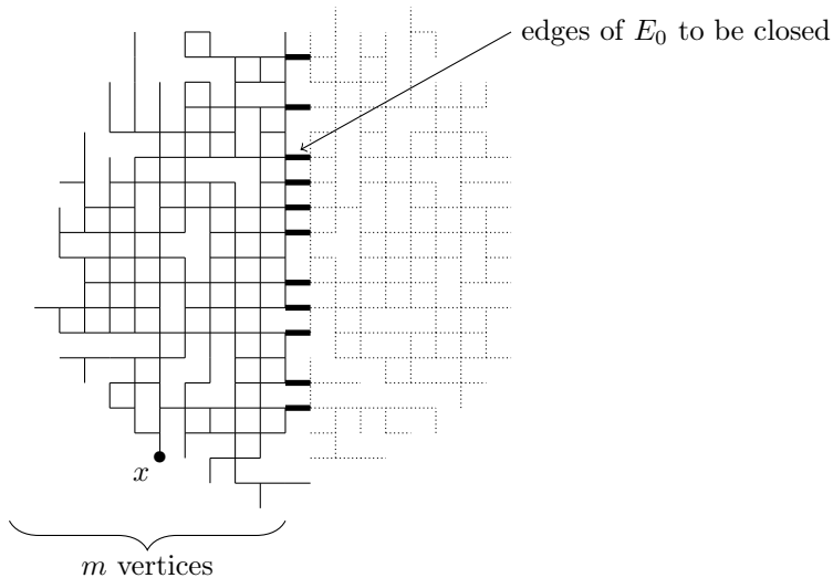
Figure 3: Closing the edges of E_0 (drawn in thick lines) cuts the graph in several connected components, such that x lies in a component (drawn in normal lines) containing the required number of vertices. Lemma 1 states that, in dimension 2, the subset E_0 can be chosen containing O(\sqrt{|V|}) edges.
