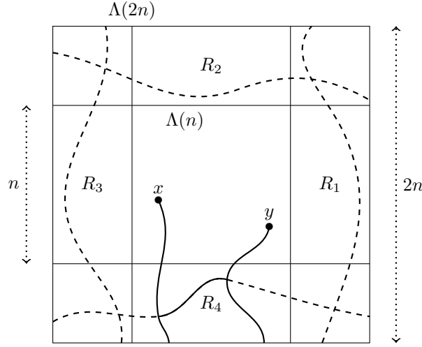
Figure 5: If each of the four rectangles is crossed by an open path in its long direction, then \Lambda(n) is surrounded by an open path in \Lambda(2n) , and thus any two vertices x and y in the box \Lambda(n) cannot be connected to \partial\Lambda(2n) without being connected to each other by an open path inside \Lambda(2n) .
