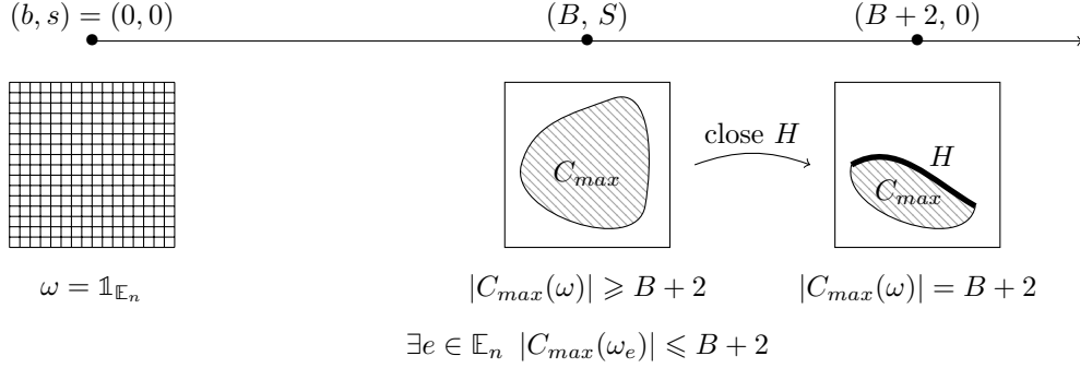
Figure 6: Sketch of the proof: if \mathcal{E} occurs, i.e., between the instants (B, S) and (B + 2, 0) , the edges H are closed but no other edges of C_{max} is closed, then the largest cluster in the configuration \omega(B + 2, 0) contains B + 2 vertices.
