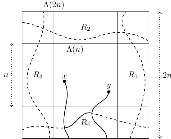
Figure 6: If each of the four rectangles R_1, R_2, R_3, R_4 is crossed by an open path in its long direction, then \Lambda(n) is surrounded by an open path in \Lambda(2n) , and thus any two vertices x and y in the box \Lambda(n) cannot be connected to \partial\Lambda(2n) without being connected to each other by an open path inside \Lambda(2n) .
