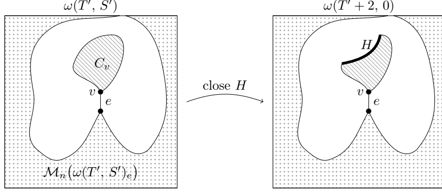
Figure 9: If (29) is a strict inequality, then closing the edge e in the configuration \omega(T', S') changes the number |\mathcal{M}_n| of vertices connected to the boundary of the box. This means that one end of the edge e , say v , happens to be disconnected from the boundary when e is closed. We then choose a subset H of the edges of the cluster C_v which is disconnected by the closure of e , such that closing all the edges of H and no other edges of \mathbb{E}[\mathcal{M}_n] between (T', S') and (T' + 2, 0) implies |\mathcal{M}_n(\omega(T' + 2))| = T' + 2 .
