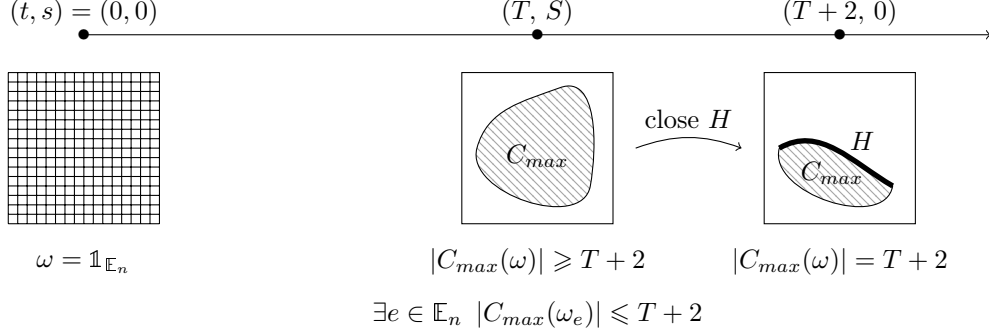
Figure 7: Sketch of the proof: if \mathcal{E} occurs, i.e., between the instants (T, S) and (T + 2, 0) , the edges H are closed but no other edges of C_{max} is closed, then the largest cluster in the configuration \omega(T + 2, 0) contains T + 2 vertices.
