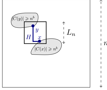
Figure 10: If there is no cluster with size \geq 2n^b , we reconstitute one by joining two clusters of size at least n^b , with a path using less than dL_n edges.
