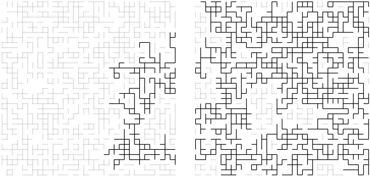
Figure 2: Percolation in the box \Lambda(35) with, left, p = 0.48 and right, p = 0.52 . Open edges belonging to the largest cluster are drawn in solid lines, while other open edges are in dotted lines.
