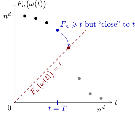
Figure 1: The partition function Z_n may be expressed as the probability that the random function t \mapsto F_n(\omega(t)) admits a fixed point. This allows for the construction of a scenario where we can force such a fixed point to appear, with a reasonable probabilistic cost.
