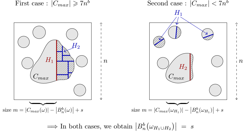
Figure 11: First case: when |C_{max}| \geq 7n^b (picture on the left), we cut a piece of C_{max} with the desired size m (by closing H_1 ) and we divide the remaining part of C_{max} into pieces smaller than n^b (by closing H_2 ). Second case: when |C_{max}| < 7n^b (picture on the right), we cut some intermediate clusters (by closing H_1 ) and we cut a piece of C_{max} with the desired size m (by closing H_2 ). In both figures, the hatched region is B_n^b(\omega) \setminus B_n^b(\omega_{H_1 \cup H_2}) , i.e., the vertices whose cluster is no longer larger than n^b after the cutting procedure.
