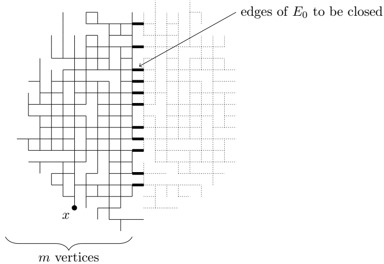
Figure 4: Closing the edges of E_0 (drawn in thick lines) cuts the graph in several connected components, such that x lies in a component (drawn in normal lines) containing the required number of vertices. Lemma 1 states that, in dimension 2, the subset E_0 can be chosen containing O(\sqrt{|V|}) edges.
