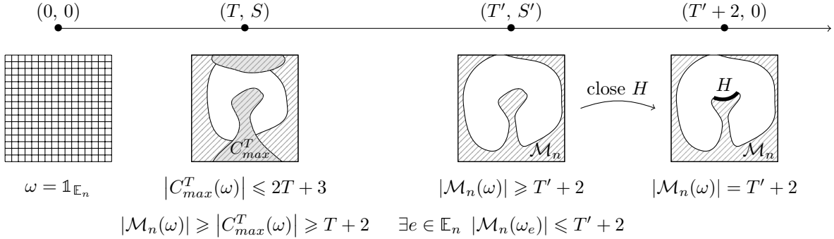
Figure 8: Illustration for the sketch of the proof of lemma 11.
