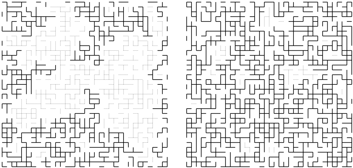
Figure 3: Percolation in the box \Lambda(35) with, left, p = 0.48 and right, p = 0.52 . Open edges connected to the boundary of the box by an open path are drawn in solid lines, while other open edges are in dotted lines.
