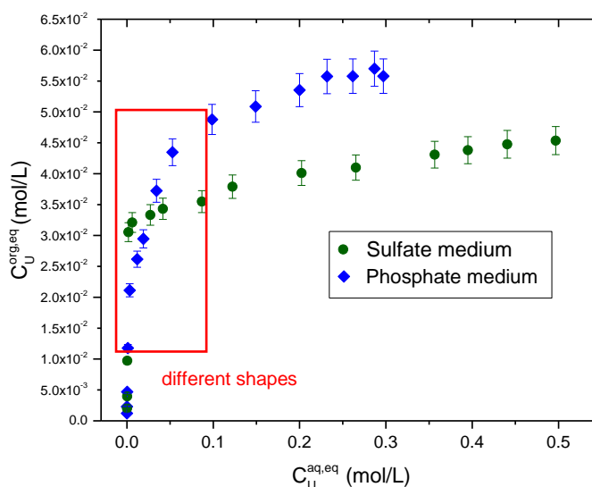
Figure 2. Uranium extraction isotherms. DEHCNPB 0.1 mol/L in TPH. Phosphate medium: [H_3PO_4] = 5 \text{ mol/L} ; sulfate medium: C_{(SO_4)_2-} = 1.6 \text{ mol/L} ; \text{pH} = 1 ; O/A = 1 ; T = 25 \text{ }^\circ\text{C} .
