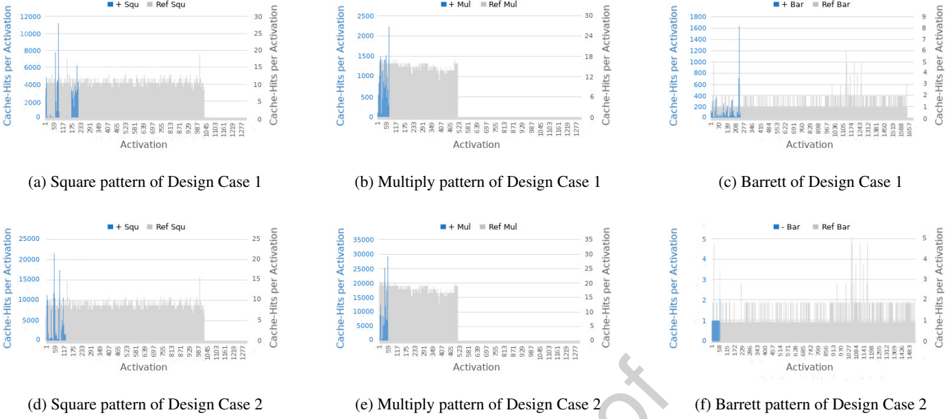
Figure 18: Activation patterns for Design Cases Design Case-1 (a)-(c) and Design Case-2 (d)-(f) +Squ. Positive noise in Square loop, +Mul: Positive noise in Multiply loop, +Bar: Positive noise in Barrett loop, and -Bar: Negative noise in Barrett loop
