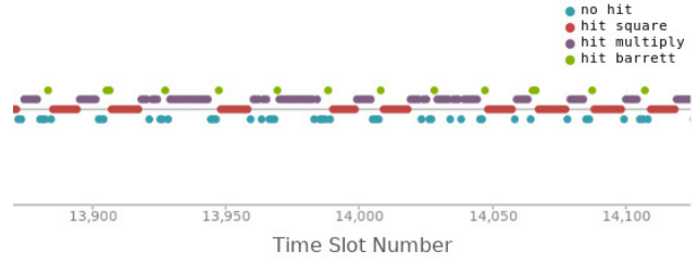
Figure 11: Graphical representation of cache access pattern without noise.
