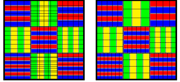
Fig. 1. Plate reactor conforming mesh (left) with 390 cells and non-conforming mesh (right) with 212 cells.
