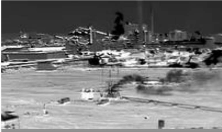
Figure 13—images obtained from the FLIR GF320 during a gas release
