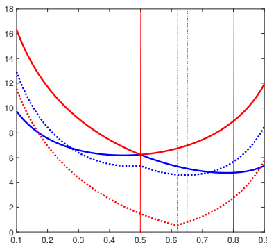
Fig. 7. Loss functions and optimal predictions of \theta (minima of the losses indicated by vertical lines) in the case of coin tossing with observations 0, 0, 1, 1, 1, 1, ?, ?, ?: solid blue line for OSL, dashed blue for the regularized OSL version (14) with \pi the beta(5,5) distribution, solid red for PSL, and dashed red for the adjusted PSL (20).
