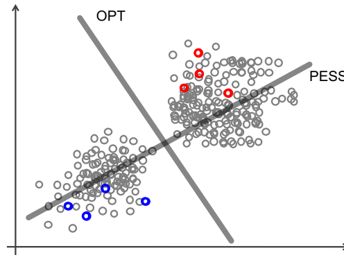
Fig. 4. Logistic regression in a semi-supervised setting: Solutions for OPT and PESS.
