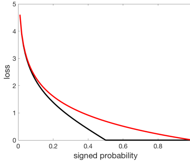
Fig. 6. The adjusted OSL version (19) of the logistic loss (black line) compared to the original version (red line).
