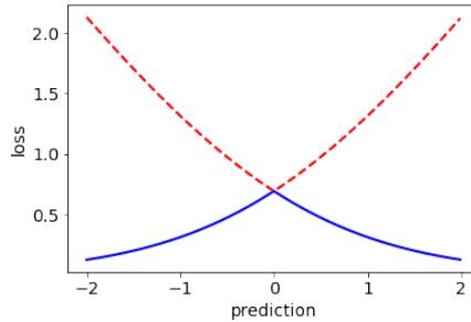
Fig. 3. OSL (blue, solid line) and PSL (red, dashed line) for the logistic loss function.
