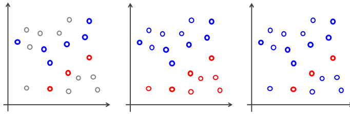
Fig. 5. Coarse data (left) together with two instantiations (middle and right).
