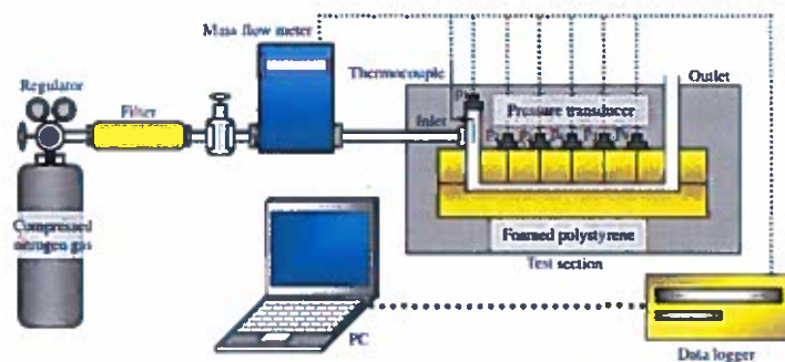
Figure 1: Schematic of experimental setup
