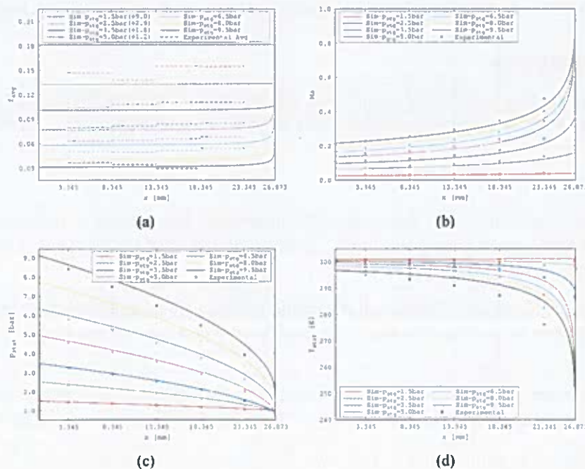
Figure 2: Comparison between 1D numerical model and experiments for MC: local/semi-local friction factor (a), local Mach number (b), local pressure (c), and local temperature (d).
