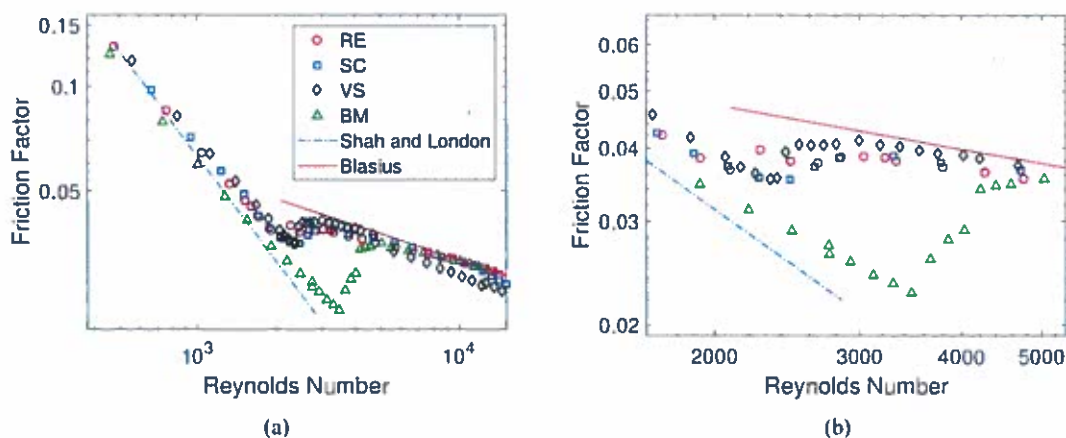
Figure 5: Comparison of f_f curves for all the tested inlet shapes to establish Re_c (a), and zoomed view in the range of 1500 < Re < 5000 (b).
