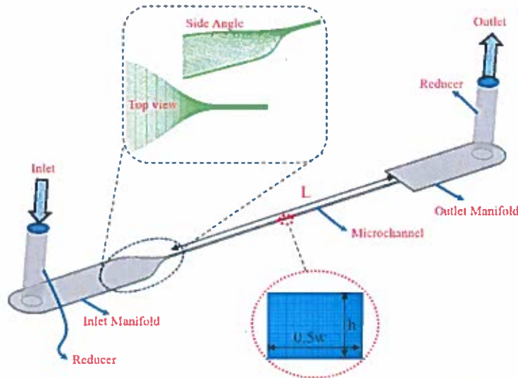
Figure 2: Geometric model used for numerical analysis of MC with bellmouth (BM) inlet.
