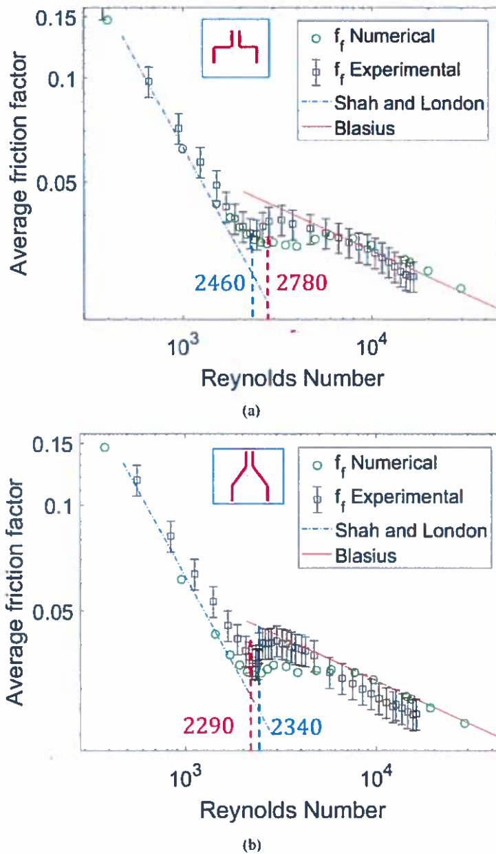
Figure 3: Friction factor for SC (a), and VS (b): blue and red vertical lines denote experimental and numerical Re_c respectively.
