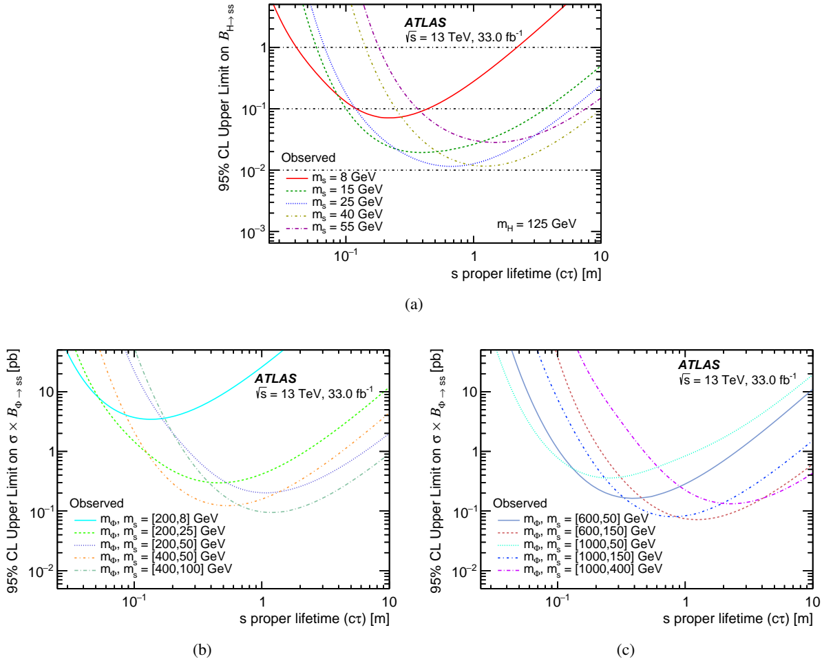
Figure 4: \text{CL}_S upper limits at 95% CL on the branching ratio B_{H \rightarrow s\bar{s}} for (a) m_H = 125 GeV, and on the cross section times branching ratio \sigma \times B_{\phi \rightarrow s\bar{s}} for (b) m_\phi = 200 - 400 GeV, and (c) m_\phi = 600 - 1000 GeV.
