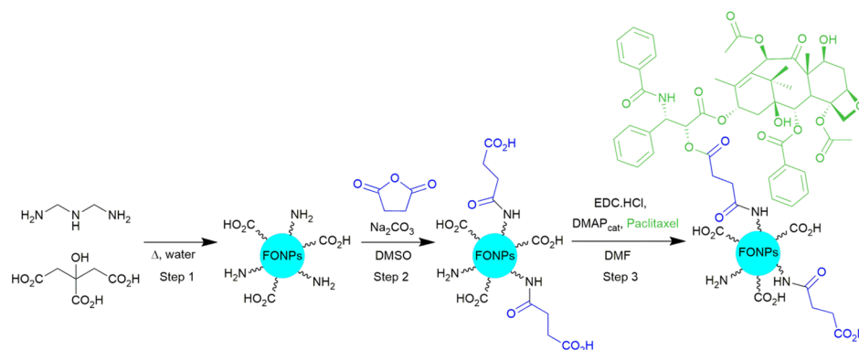
Scheme 1. Synthesis Steps of the FONP–PTX Prodrug a
