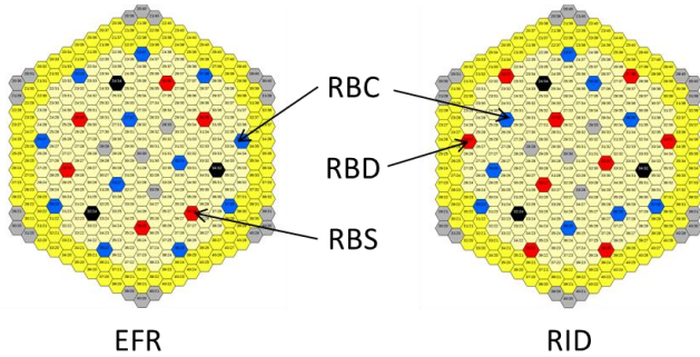
Fig. 3. Positions of RBC, RBD and RBS in RID and EFR architecture
