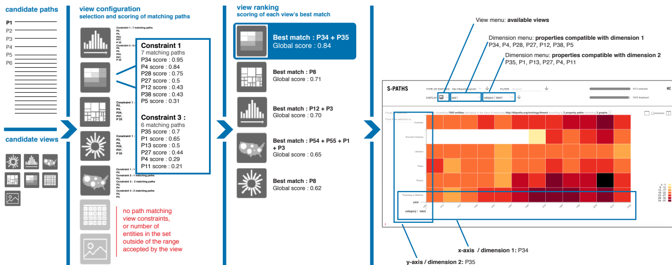
Figure 2: S-Paths' process for generating a default view.
