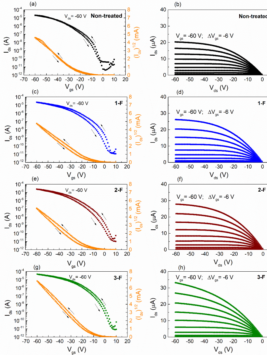
Figure 4. Transfer (a) and output (b) characteristics of the devices on bare \text{SiO}_2 (non-treated); those of the devices treated with phenylboronic acid molecules: 1-F (c) and (d); 2-F (e) and (f); 3-F (g) and (h).
