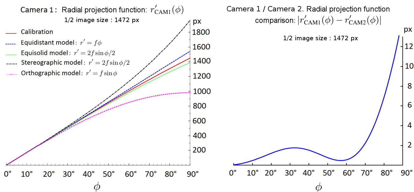
Figure 6. Left figure : radial projected distance r' as a function of incident angle \phi for VIVOTEK camera 1. Function r'(\phi) is called representation function as it characterizes the projection. It is compared to the mostly used fisheye parametric representation functions set with -a_0 value for f . Right figure : difference in pixels between representation functions of camera 1 and camera 2, as a function of incidence angle \phi .
