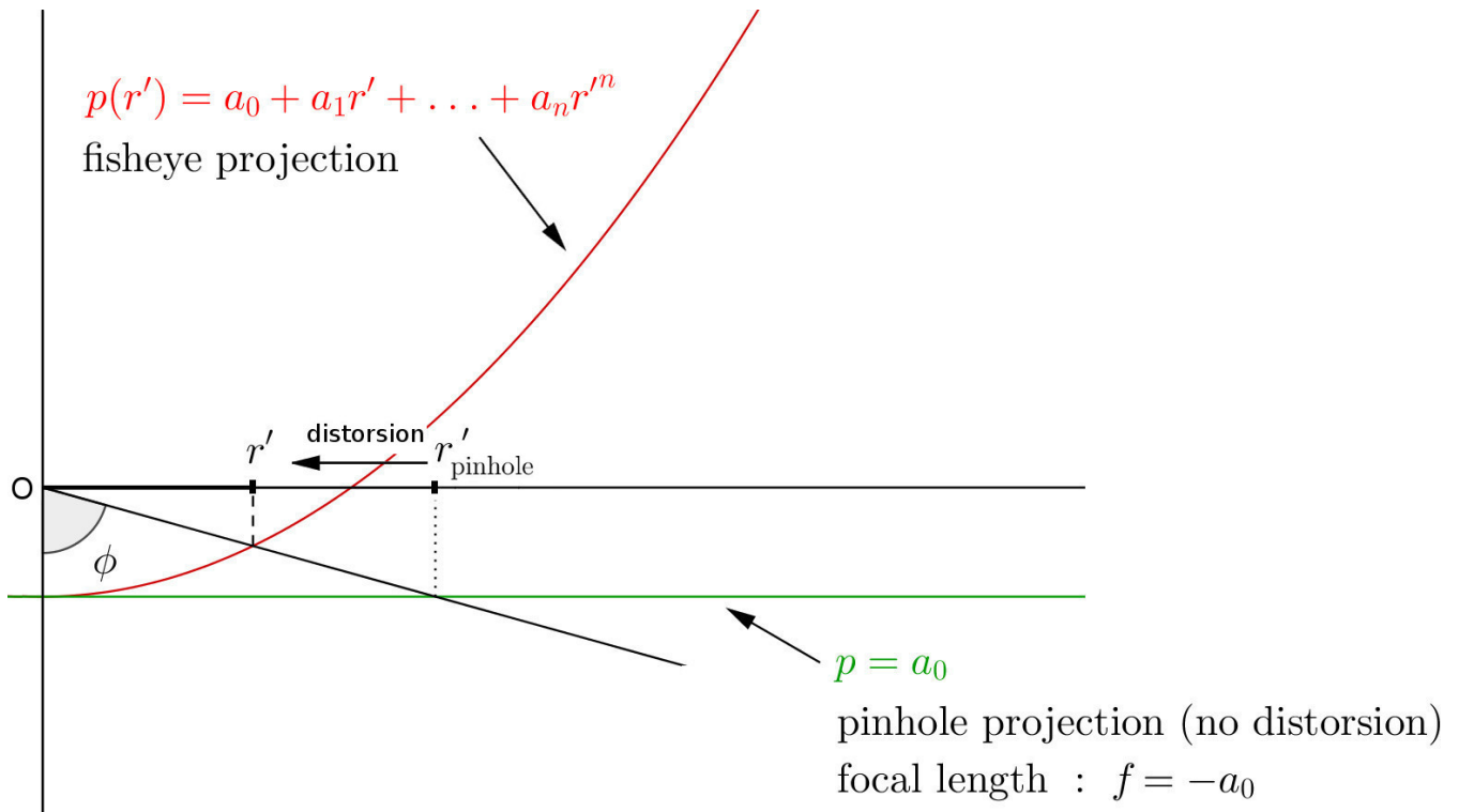
Figure 2. Radial distortion modelization in Scaramuzza et al. (2006) for omnidirectional cameras. Incident angle \phi and projected radial distance r' are related by \tan \phi = -r'/p(r') . The polynomial function p is represented by the red curve. The case where there is no distortion (i.e. pinhole projection r' = f \tan \phi ) corresponds to a constant polynomial function p = a_0 represented by the green line.
