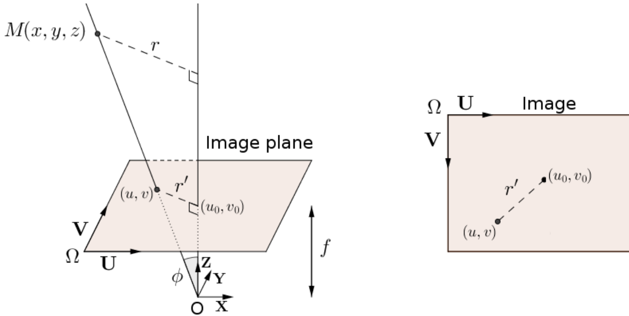
Figure 1. Pinhole projection. Physical point M is projected on (u, v) on the image-plane (\Omega, U, V) . Camera coordinate system is defined by axis X and Y which are colinear to U and V , and by axis Z which is the optical axis . Principal point (u_0, v_0) is the projection of the optical center O on the image. The radial projected distance on the image is denoted r' .
